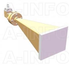
LB-12-25-C-1.0FSPO Standard Gain Horn Antenna 60-90GHz 25dB Gain 1.0mm Female
